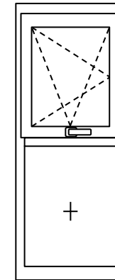
Code 2.16: Tilt & Turn, Fixed. Transom
