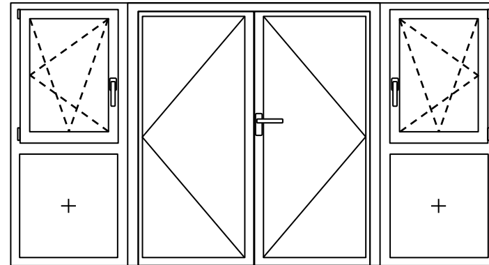
Code 7.10: OW French, 2 x Tilt & Turn Sidelights with Transoms
