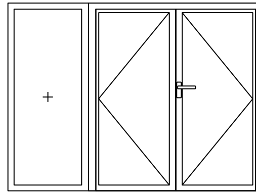
Code 7.12: OW French, Sidelight
