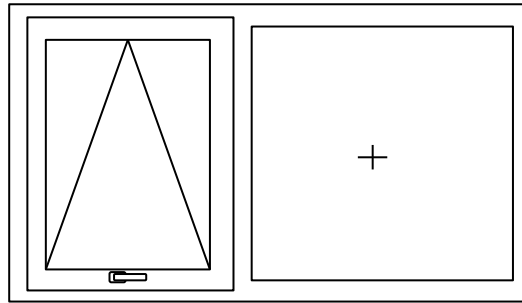
Code 3.05: Awning, Fixed
