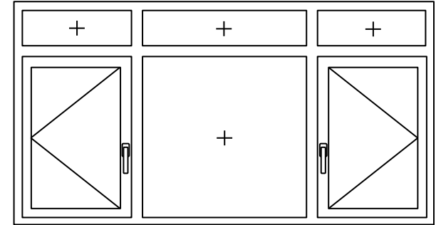
Code 3.03: 2 x Casement, 3 x Fixed
