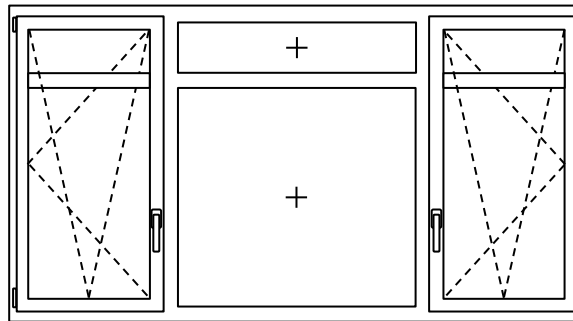
Code 2.06: 2 x Tilt & Turn, 2 x Fixed
