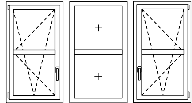
Code 2.13: 2 x Tilt & Turn Bay Window
