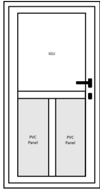
Code 6.17: 2 x Panel, Glass
