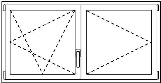
Code 2.08: Tilt & Turn, Turn. No mullion
