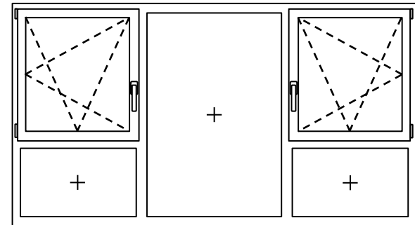
Code 2.07: 2 x Tilt & Turn, 3 x Fixed
