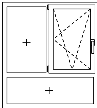
Code 2.14: Tilt & Turn Centre Hinge, 2 x Fixed
