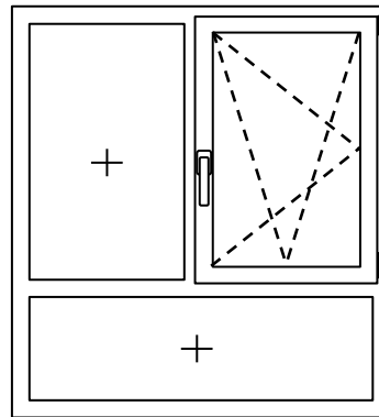
Code 2.15: Tilt & Turn, 2 x Fixed
