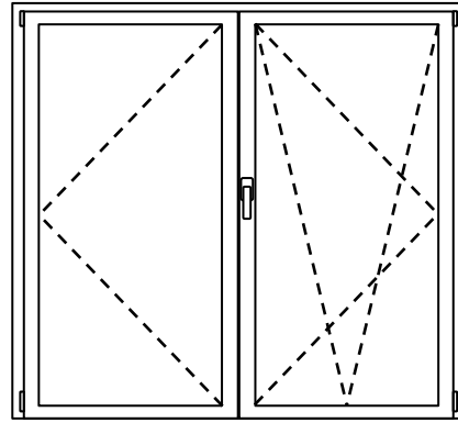
Code 7.07: IW French Tilt & Turn
