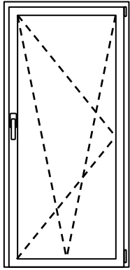
Code 7.01: IW Tilt & Turn
