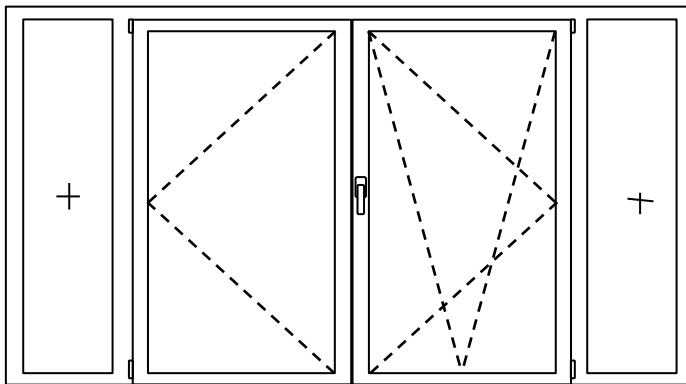
Code 7.13: IW French, 2 x Sidelights
