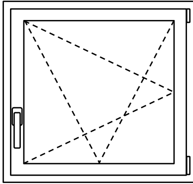
Code 2.01: Single Tilt & Turn
