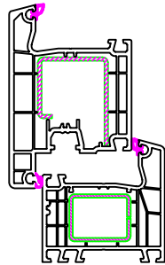
140x07 & 140x31 Frame & Sash • Outward opening door
