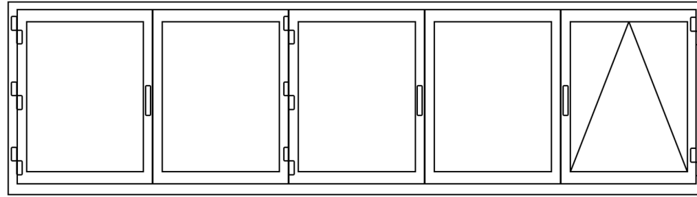
Bi-fold 541 (with tilting main window)
